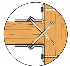
Double Shear Nailing.
